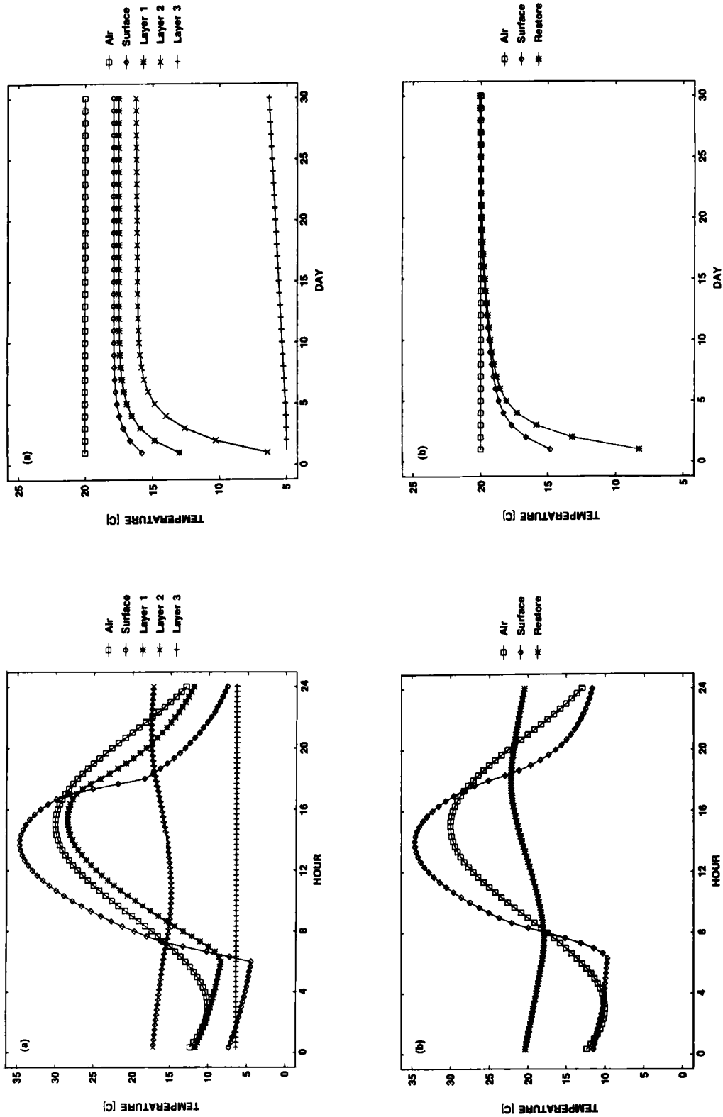
Figure 4. Run 1—Soil and air temperatures for the last day: (a) CLASS; (b) old scheme
