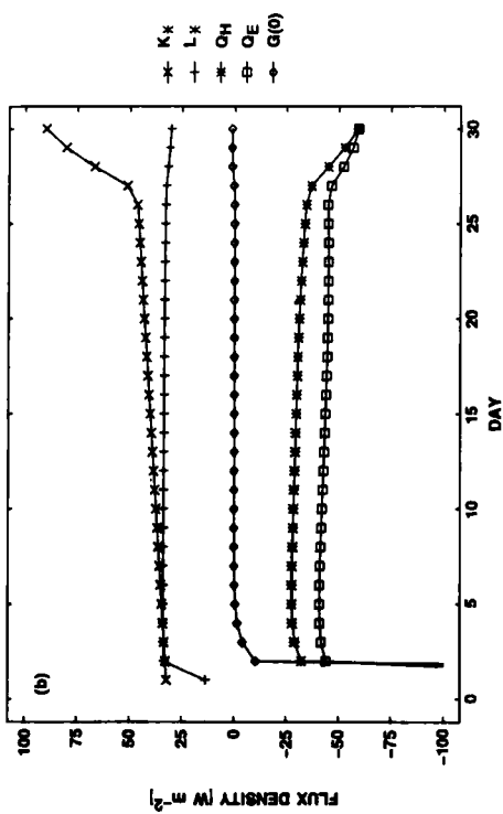
Figure 11. Run 3—Daily average energy balance terms: (a) CLASS; (b) old scheme
